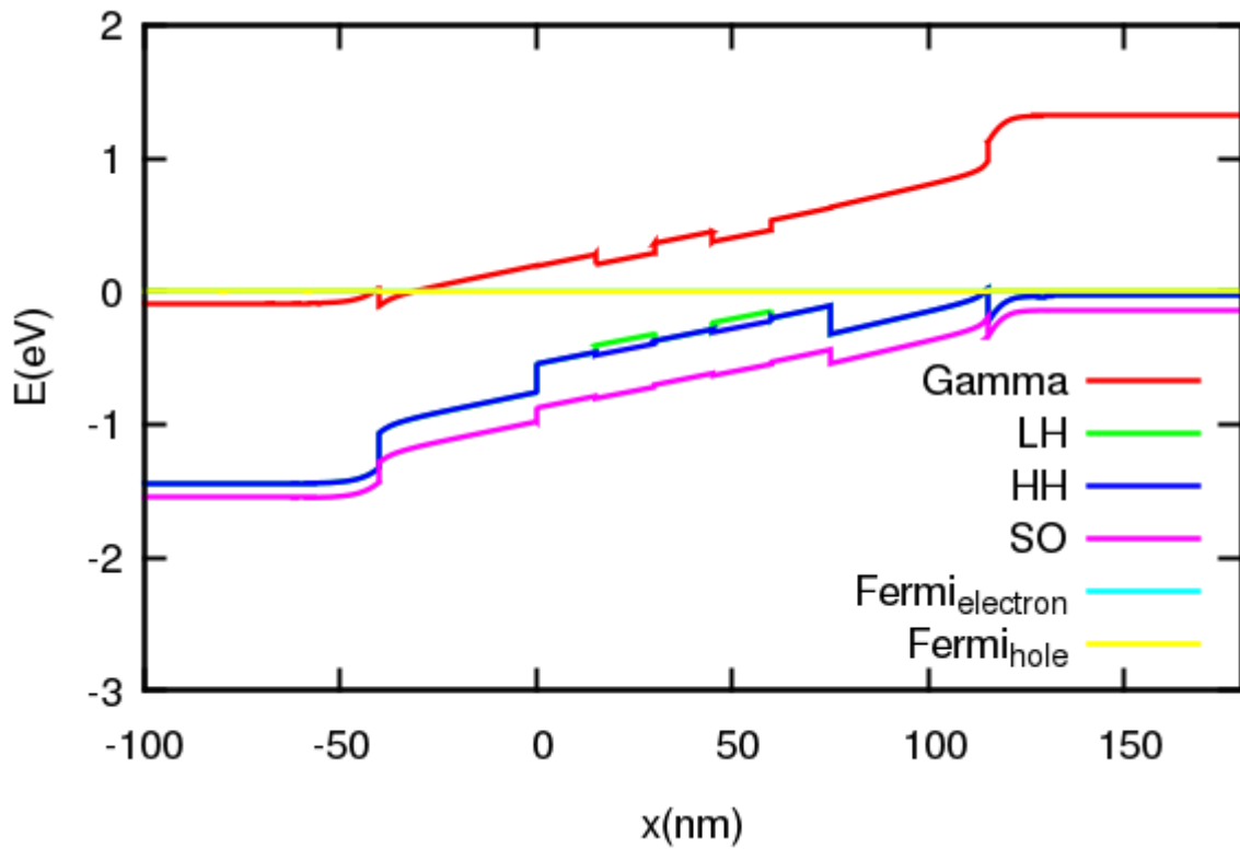
Figure 1: Bandstructure with zero bias. Two Quantum wells with alloy structures \text{In}(0.7)\text{Ga}(0.3)\text{As} , and well barriers \text{In}(0.53)\text{Ga}(0.47)\text{As}
