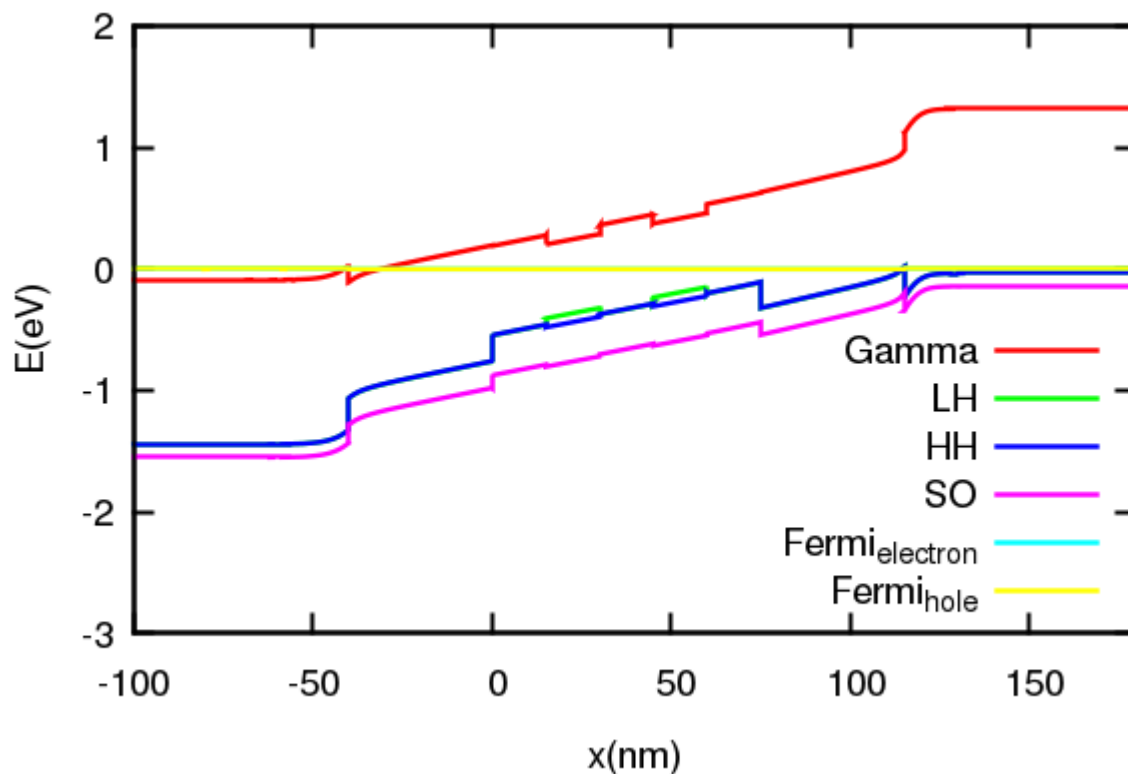
Figure 1: Bandstructure with zero bias. Two Quantum wells with alloy structures In(0.7)Ga(0.3)As , and well barriers In(0.53)Ga(0.47)As
