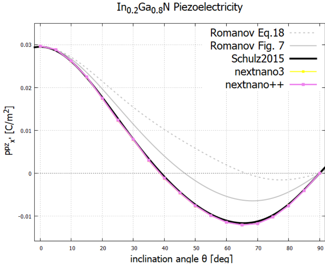
Figure 6: Piezoelectric polarization as a function of inclination angle. The gray curve is the analytical result of Eq. (18) in [Romanov2006], i.e. the curve (4) in Fig. 7(a) where the factor 2 is missing.
